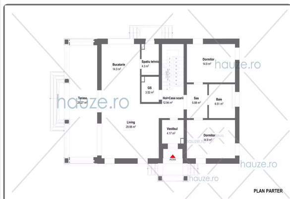
Plan Parter - 136.77mp
