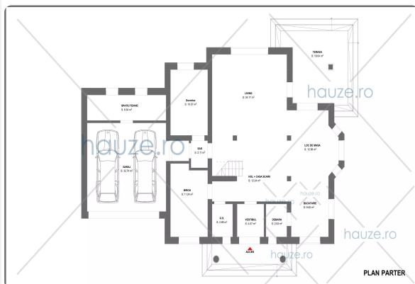
Plan Parter - 143.8mp
